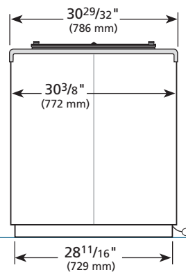
RIGHT VIEW
