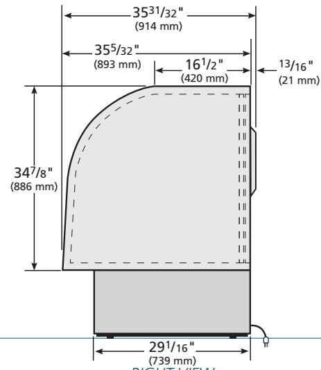
RIGHT VIEW
