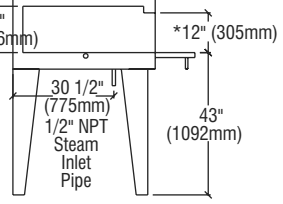
ER-12-5736 SIDE VIEW
