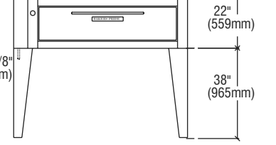
ER-12-5736 FRONT VIEW
