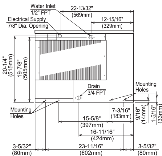
AIR-COOLED UNIT
