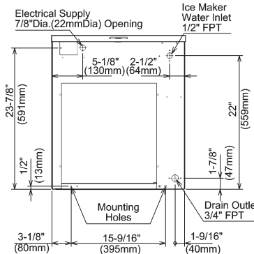
AIR-COOLED UNIT
