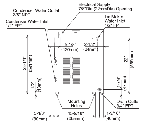
WATER-COOLED UNIT
