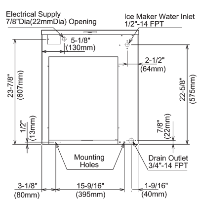
AIR-COOLED UNIT
