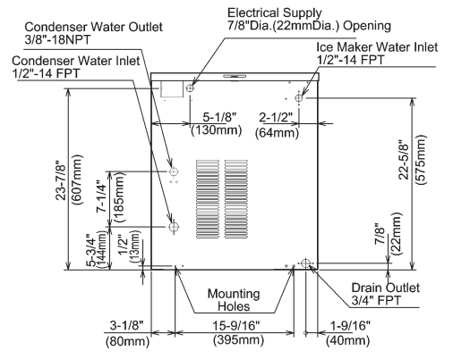
WATER-COOLED UNIT
