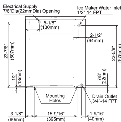
AIR-COOLED UNIT
