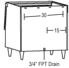
3/4" FPT Drain
