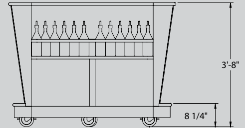
BACK VIEW
