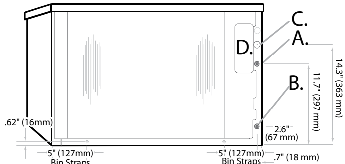
Air Cooled
