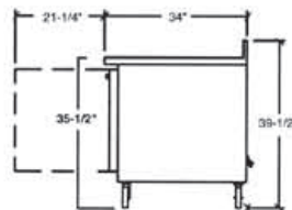
WTR46, 67, 93, 119, WTF67 Common End View
