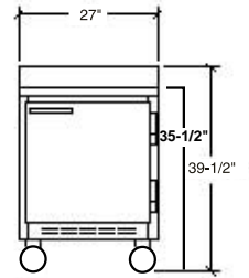
WTR27 Front
