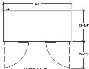
WTR60 Top
