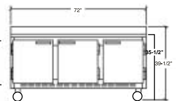
WTR72 Front
