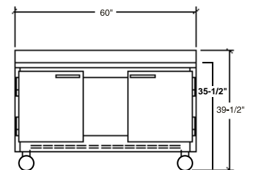
WTR60 Front
