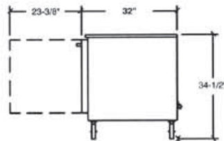
UCR46, 67, 93, 119 UCF67 Common End View
