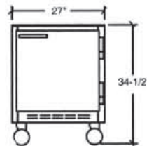
UCR-27SD Front
