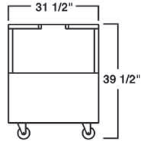
ST34N, 49N, 58N Common End View
