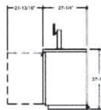
DD50, 58, 68, 78, 94 Common End
