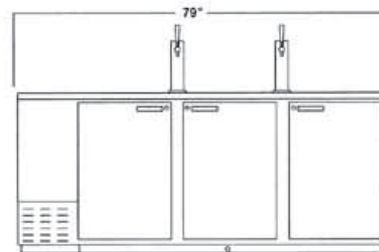
DD78 Front
