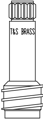
000800-25 RIGHT HAND SPINDLE ( 1 SUPPLIED )
