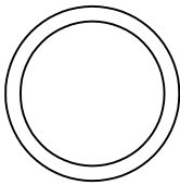
001062-45 O-RING 11/16" I.D. [17mm] 3/4" O.D. [19mm] ( 2 SUPPLIED )
