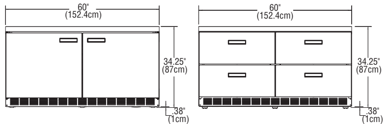
ELEVATION VIEW UC4460N
