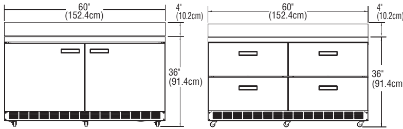
ELEVATION VIEW ST4460N
