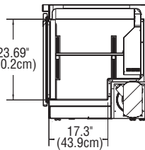
END VIEW UC4460N
