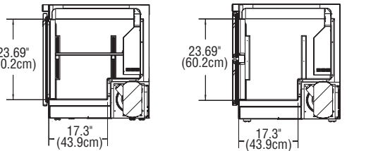
END VIEW UC4460N
