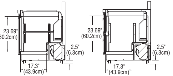
END VIEW ST4460N
