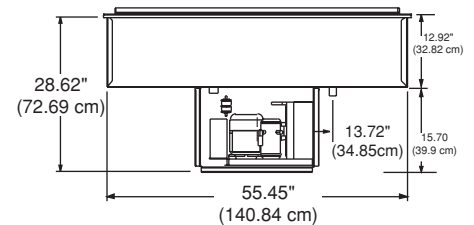
ELEVATION VIEW N8157-FA
