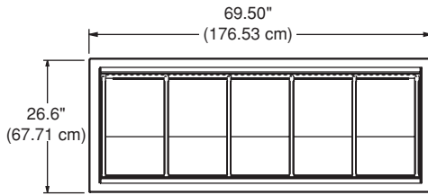
PLAN VIEW N8169-FA
