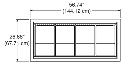
PLAN VIEW N8157-FA
