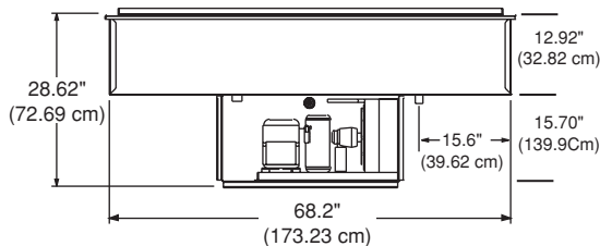
ELEVATION VIEW N8169-FA
