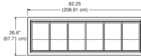
PLAN VIEW N8182-FA
