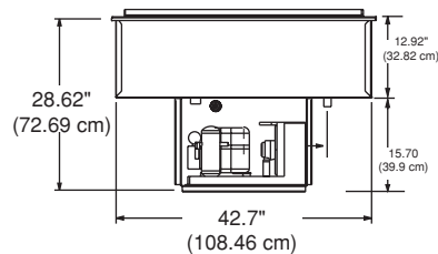
ELEVATION VIEW N8144-FA
