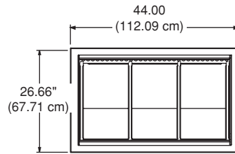
PLAN VIEW N8144-FA
