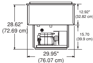
ELEVATION VIEW N8131-FA
