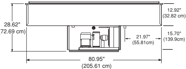
ELEVATION VIEW N8182-FA
