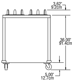
ELEVATION VIEW CAB4 MODELS
