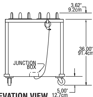
ELEVATION VIEW CAB4-ET & CAB4-QT MODELS
