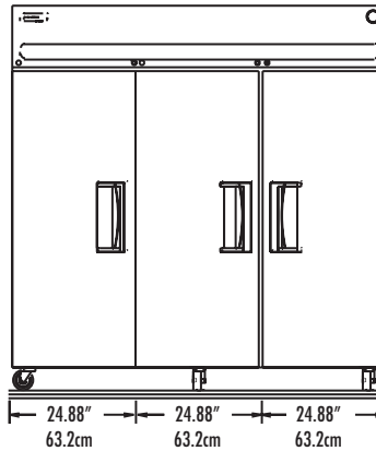
Elevation View 6076XL-S and 6076XL-SR
