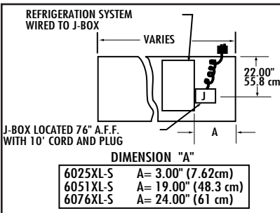
Mechanical Detail
