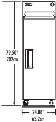
Elevation View 6025XL-S and 6025XL-SR
