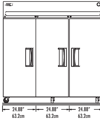
Elevation View 6076XL-S and 6076XL-SR
